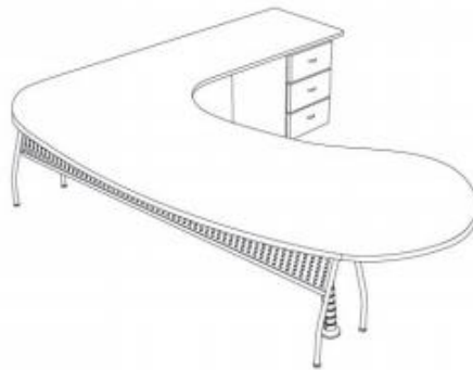
N-3 "L" Shape Workstation 1800(W) x 1800(D) x 750(H)
