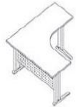
'L' SHAPE EXECUTIVE TABLE SW-08 : 1200W x 1500W x 600D x 750H SW-09 : 1500W x 1500W x 600D x 750H SW-10 : 1800W x 1800W x 700D x 750H SW-11 : 1800W x 1500W x 700D x 750H
