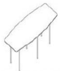
CONFERENCE MEETING TABLE SW-19 : 1800W x 1050D x 900D x 750H SW-20 : 2100W x 1050D x 900D x 750H SW-21 : 2400W x 1050D x 900D x 750H
